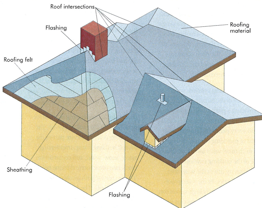
FIGURE 1 ROOF SYSTEM COMPONENTS
